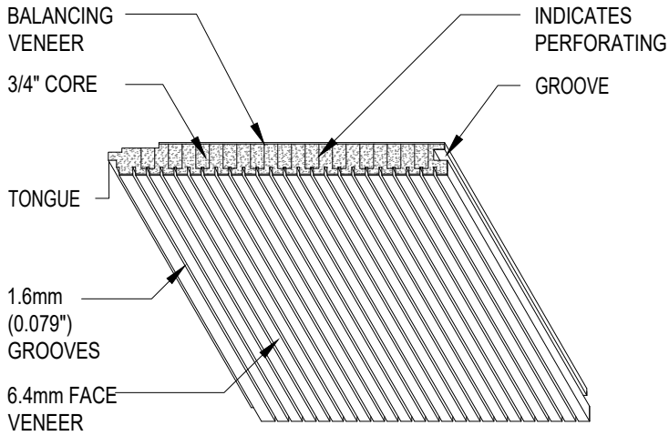
1 AUDITION PLANK PROFILE SCALE: 3" = 1'-0"
