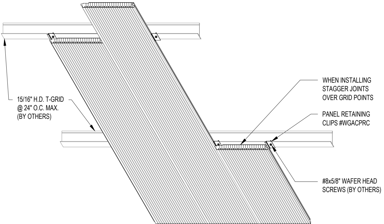
3 CEILING PLANK MOUNTING SCALE: 1 1/2" = 1'-0"
